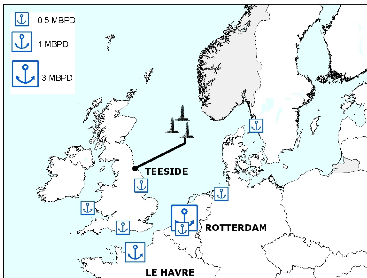
Figure 5 Norpipe Pipeline
